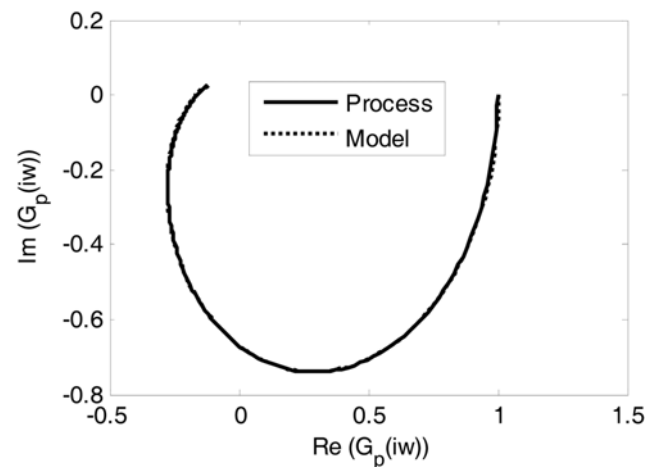
Fig. 7. Identification results of the proposed method for the initial-unsteady-state process.
