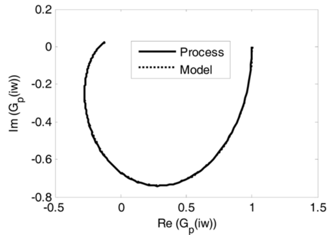
Fig. 6. Identification results of the proposed method for the initial-steady-state process.
